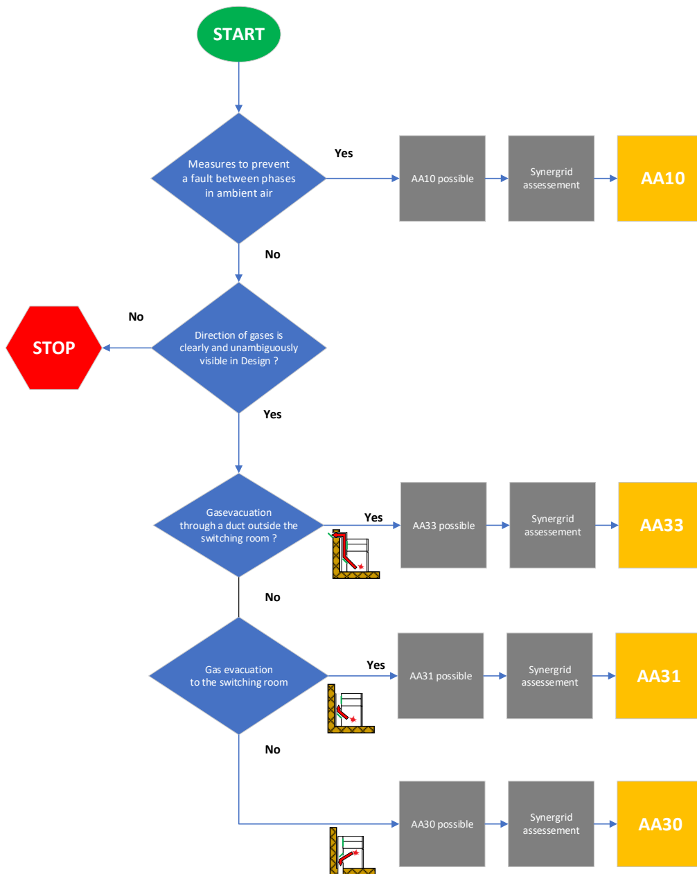
Figure 2: Flowchart for the assignment of an AA category of the HV metering functional units
